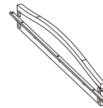
Ref: D Double:1656x275mm King:1736x275mm Superking:1736x275mm Quantity: 2
